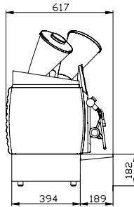
Schaerer Coffee Celebration BCL Kaffee, Heisswasser, Dampf, Milch Coffee, Hot Water, Steam, Milk
